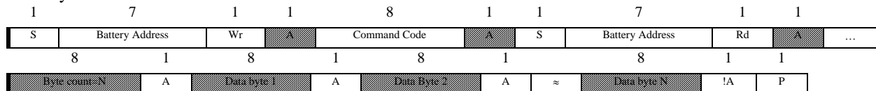
Block Read
